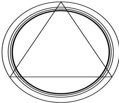
Fig. 2.1 Convergence to Finiteness
