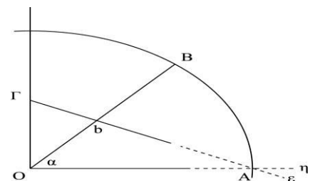
Fig.4.4.The Euclidean Axiom
