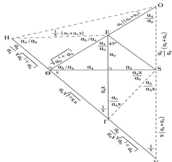
Fig.4.2. Construction of Quartic Equation Roots
