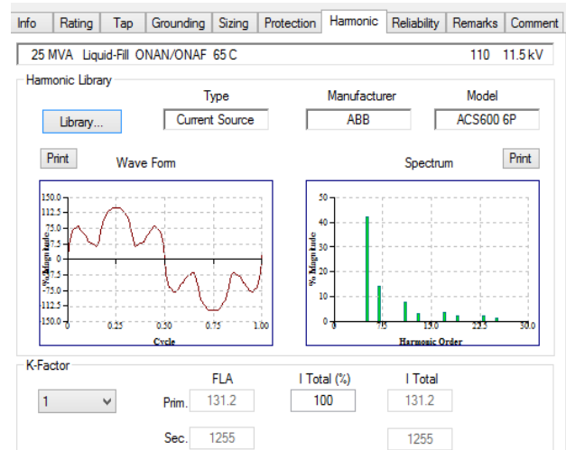
Fig. 10. Harmonics in the grid
