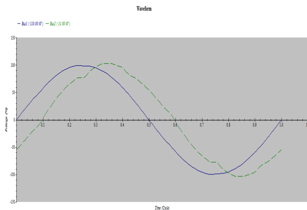
Fig. 9. No Harmonics waveform in bus 1 & bus 2
