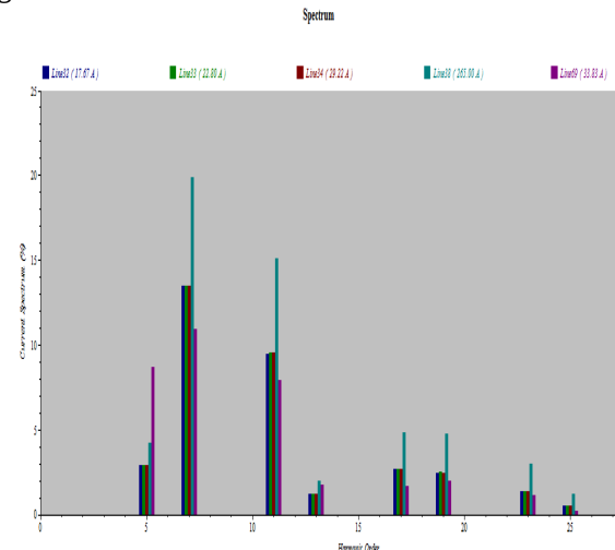
Fig. 15. Distortion current spectrum in the bus 1 & bus 2
