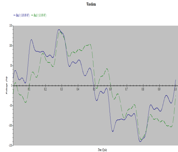
Fig. 12. Distortion voltage waveform in the bus 1 & bus 2
